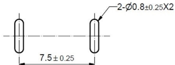
MOUNTING HOLES
